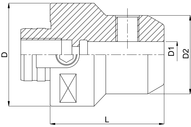
VARILOK SYSTEM
